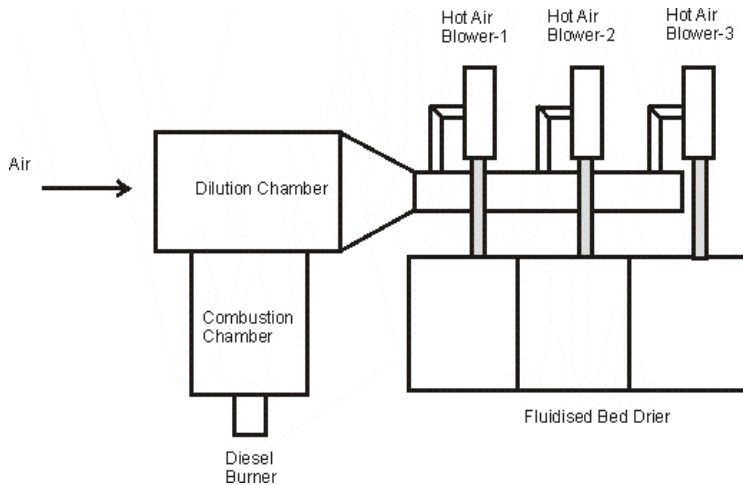
Figure 1: Schematic of the fossil fuel set up
