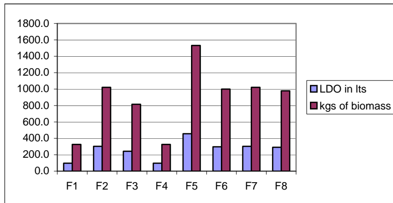
Figure 10: Fuel requirement for various furnaces
