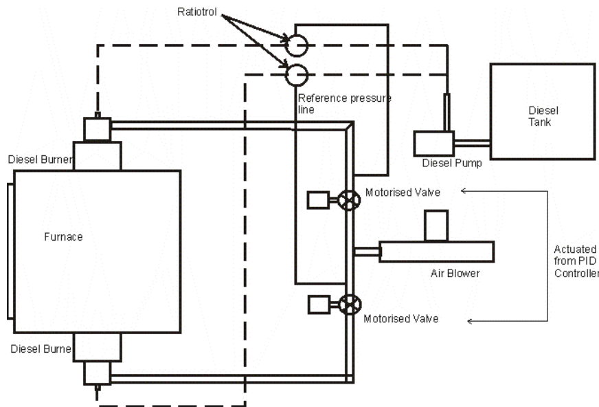
Figure 6: Fossil fuel system for high temperature application
