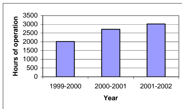
Figure 5: Hours of operation on the 200 kg/hr gasifier system
