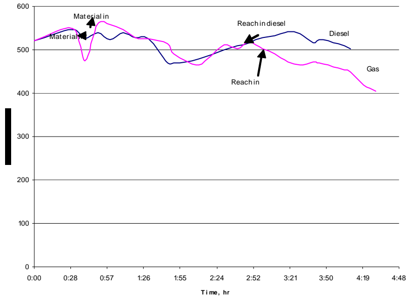
Figure 8: Comparison of temperature inside a furnace using diesel and gas
