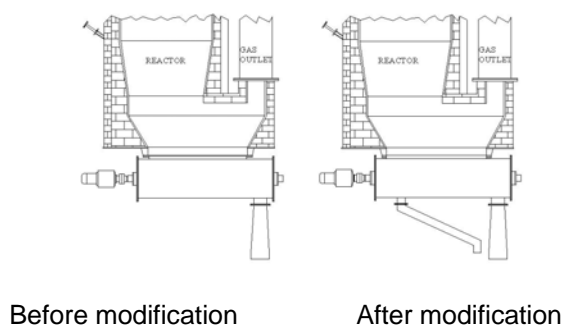
Figure 4: Changes implemented on the ash extraction system
