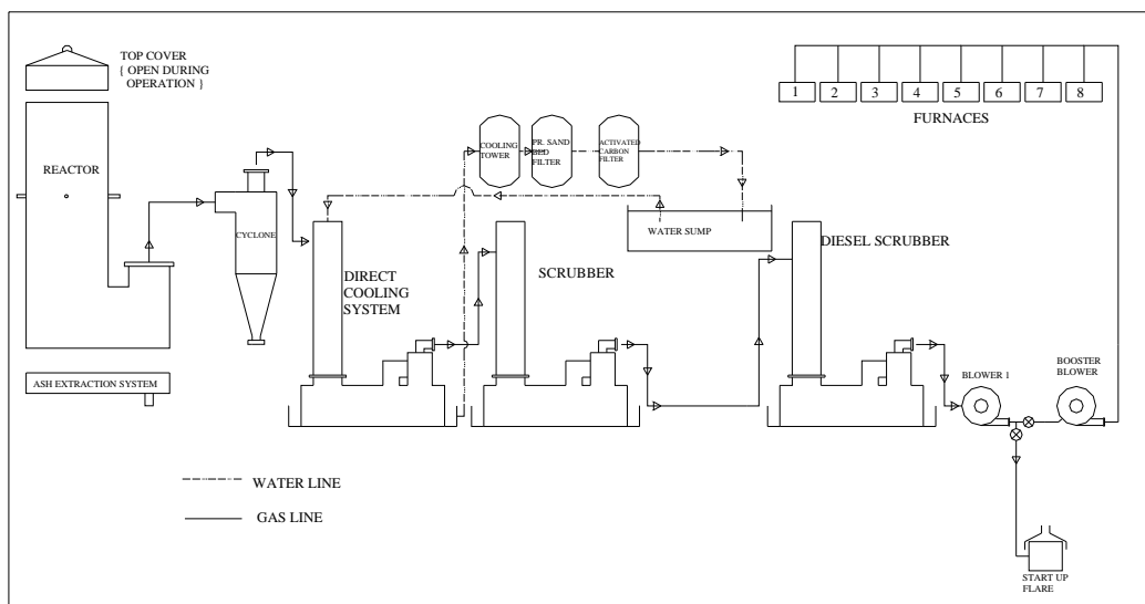
Figure 7: Schematic of the 300 kg/hr gasifier system
