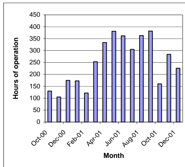
Figure 3: Hours of gasifier operation using coconut shell for various months
